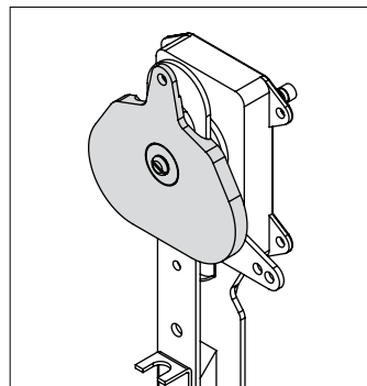
Manetta 'Push'
